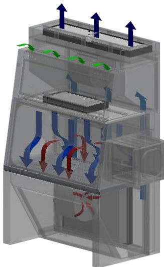
BSC Class III Airflow Diagram
